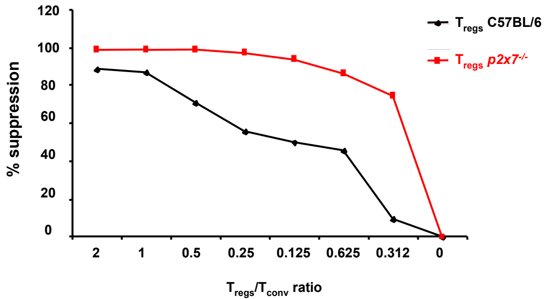
Fig. S1. Increased suppressive function by P2X7 deficient T regs . Suppression assay performed with WT (black line) or p2x7 -/- (red line) T regs and WT responder T conv cells. Cell proliferation was determined by 3 H-thymidine incorporation.
