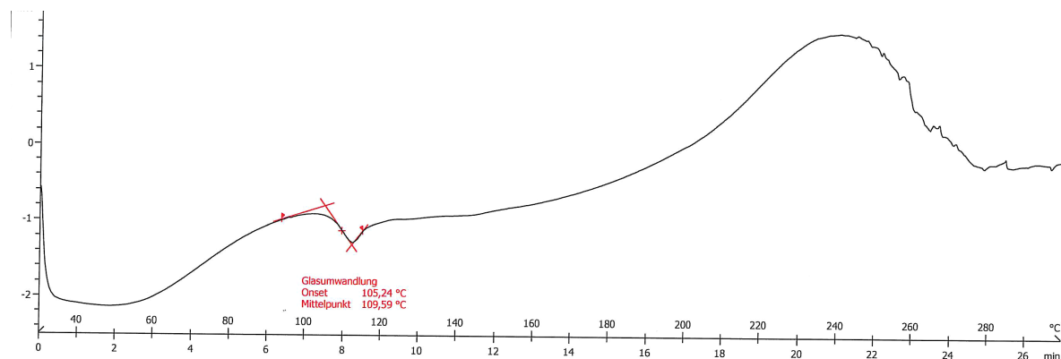
Figure S1: DSC of substance A amorphous base: glass transition point is between 6 and 10 minutes at approx. 110°C (heating rate 10°C/min)
