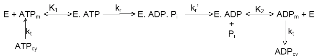
Figure 3. Kinetic Scheme for ATP Hydrolysis by F 1 -ATPase
