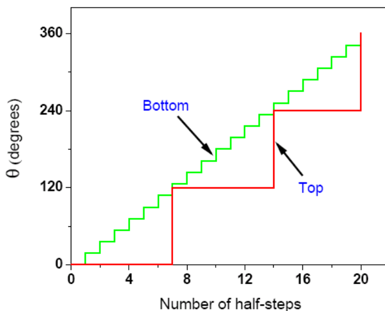
Figure 1. Torsional mechanism for F_1F_0 -ATP synthase with symmetry mismatch. The diagram is drawn for a ring of ten c-subunits ( i.e. , n=10 ) and half-steps of 360^\circ/(2n) . A symmetry mismatch between c and \gamma rotation of 6^\circ after 120^\circ , and 12^\circ after 240^\circ [for half-steps of 360^\circ/(2n) ] is found. After 360^\circ , it is found that the symmetry mismatch becomes zero.
