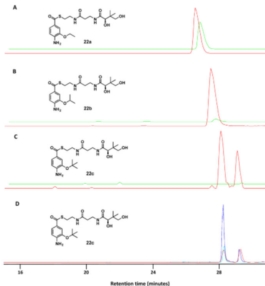
Figure 5. LC-MS analysis of CysS-catalyzed iterative methylations of methyl ether 21 . Red trace is for the complete reaction mixture. Green trace is for reaction mixtures where the reducing system (flavodoxin/flavodoxin reductase/NADPH) is absent. Ethyl ether 22a , isopropyl ether 22b were not formed in the control reactions lacking CysS, SAM, or MeCbl. (A) Extracted ion chromatograms (EICs) of the ethyl ether 22a [M+H]^+ ( 442.20 \pm 0.02 ). (B) EICs of the isopropyl ether 22b [M+H]^+ ( 456.22 \pm 0.02 ). (C) EICs of the t -butyl ether 22c [M+H]^+ ( 470.23 \pm 0.02 ). (D) EICs of [M+H]^+ ( 470.23 \pm 0.02 ) showing comigration with a synthesized sample of 22c . Cyan trace is the t -butyl ether standard. Blue trace is coelution of the enzymatic product and synthetic standard. The second component in the extracted ion chromatogram for the t -butyl ether 22c (panels C, D) was identified as the sec -butyl ether 22d (Figure S7). The product ratio was determined by calibrating signal intensity with known concentrations of standards (SI).
