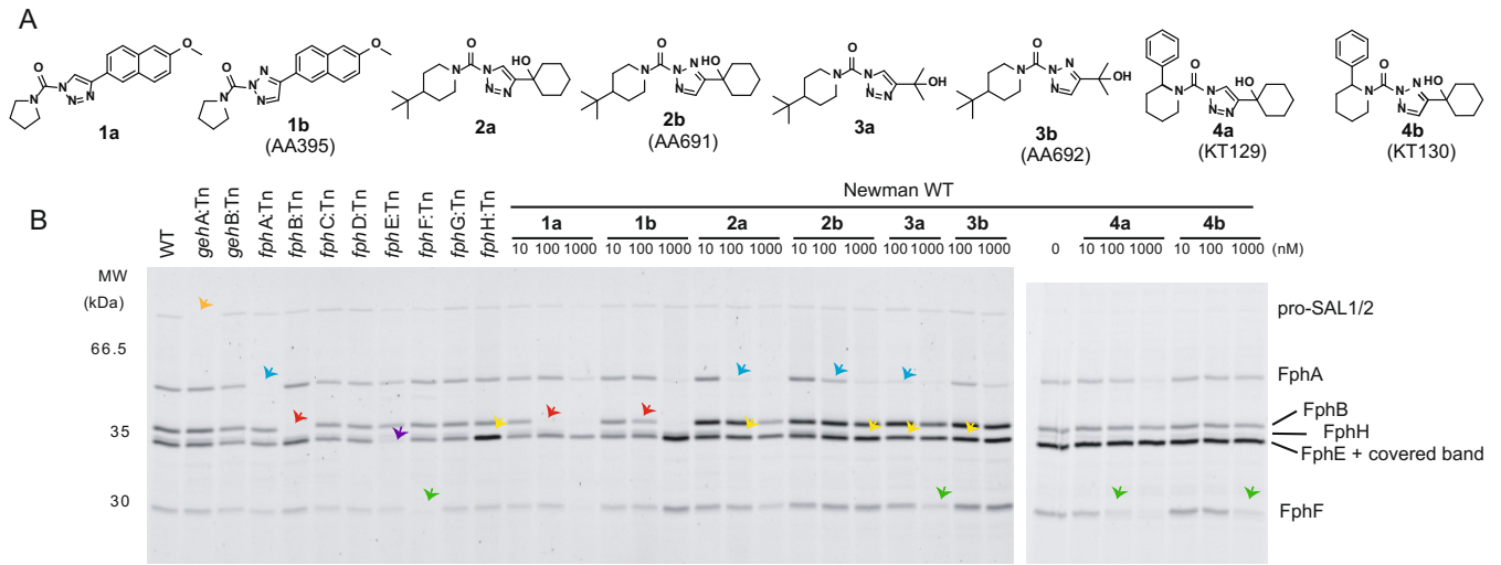
Figure 1. Inhibitory profile of TU screening hits and labeling profile of clickable probes. A) Chemical structures of hit compounds and their regioisomers 1-4 a/b . B) Competitive FP-TMR labelling profiles of S. aureus Newman WT or indicated transposon mutant (:Tn) strains after preincubation with compounds 1-4 a/b . Cells were harvested from TSAMg plates, preincubated with inhibitors for 60 min, labelled with FP-TMR (1 \mu M), lysed and analysed by SDS-PAGE/fluorescence scan. Preferred targets of each probe (according to transposon mutant analysis) are highlighted by colored arrows: Orange: SAL1, blue: FphA, red: FphB, green: FphF, yellow: FphH, purple: FphE.
