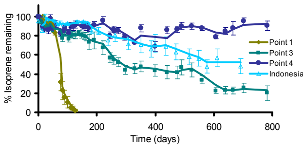
A Colne estuary and Indonesia water, 0.1% isoprene
