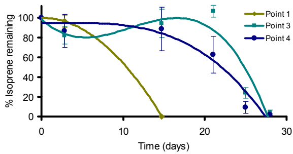
C Colne estuary water, 0.001% isoprene
